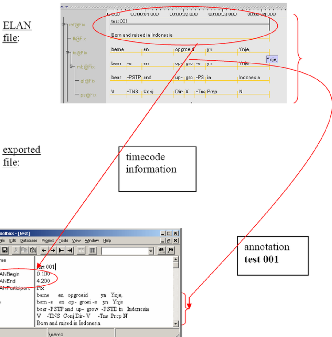
Figure 1.51. ELAN file and exported file
