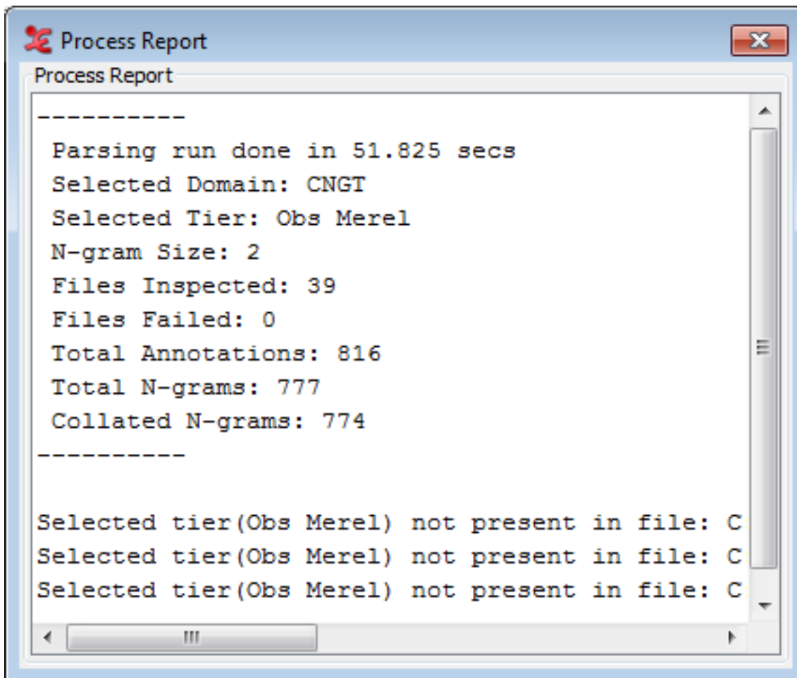
Figure 1.140. N-Gram Analysis process report
