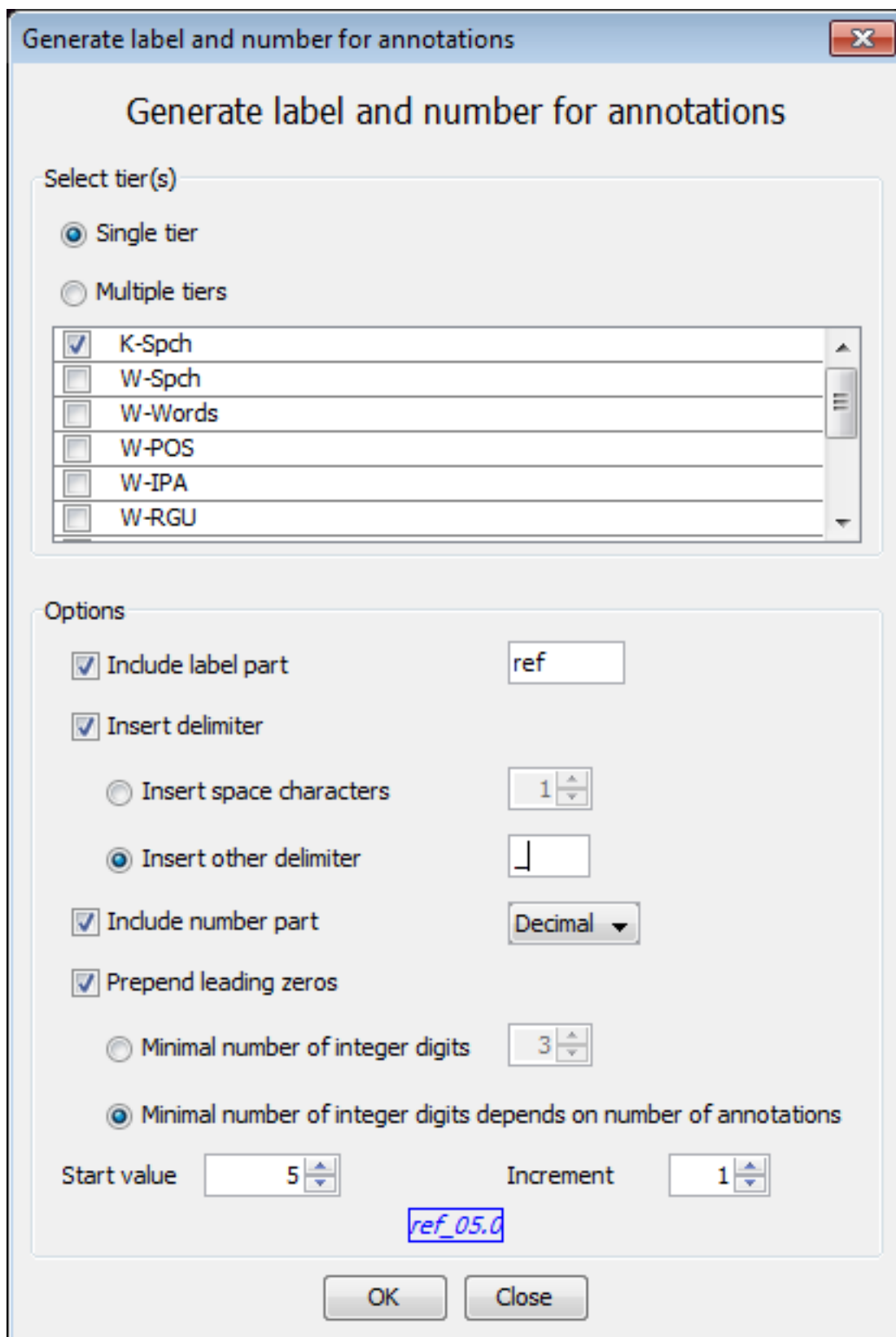
Figure 2.76. Label and Numbering annotations
